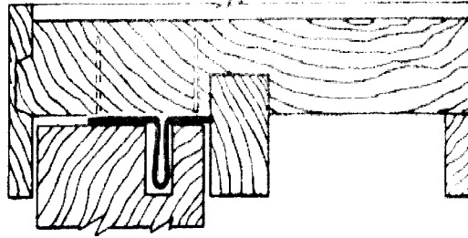
Head Section
