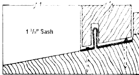
Sill Section
